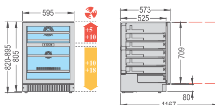
WINE 45 FG DUAL TEMPERATURE BUILT-IN & FREE STANDING
