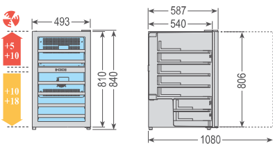
WINE 32 FG DUAL TEMPERATURE ONLY FREE STANDING
