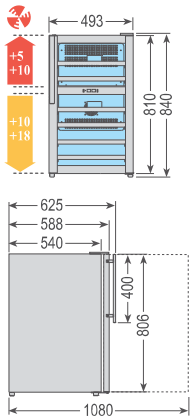
WINE 32 DUAL TEMPERATURE FREE STANDING
