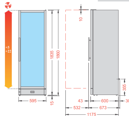
WINE 185 / WINE 185 BLACK FREE STANDING
