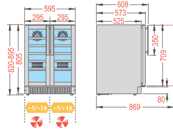
WINE 38 DUAL TEMPERATURE BUILT-IN & FREE STANDING
