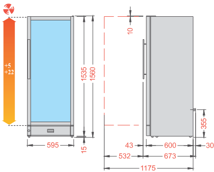
WINE 155 BLACK FREE STANDING
